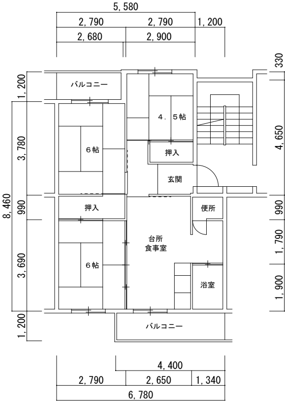
(3DK) 4~8号館 (79204-01)
