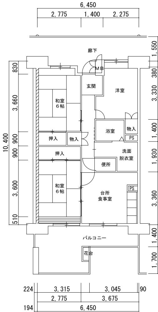
3DK a
