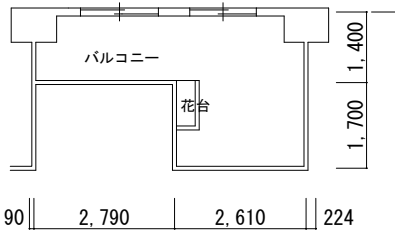
2DK b
